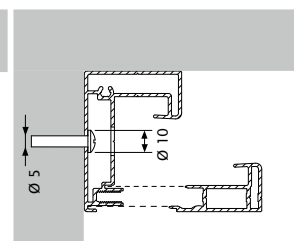
Side mounting of the side channel Fixscreen® 85
