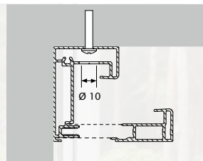
Rear mounting of the side channel Fixscreen® 150 (F)
