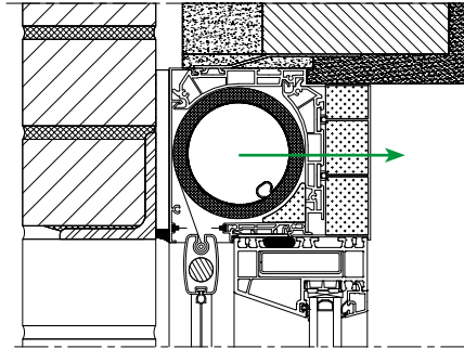
Installation method 4: Fixscreen® Mono AK Medium+
