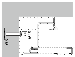
Side mounting of the side channel Fixscreen® Mono AK
