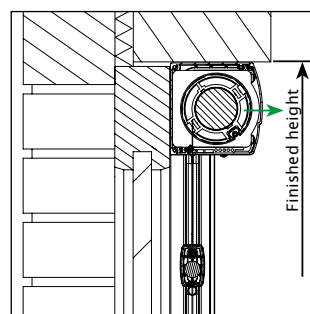
Surface-mounted, inside, in front of the window
