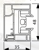
Closed side channel (G)
