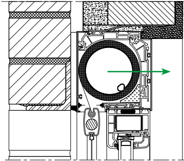
Installation method 4: Fixscreen® Mono AK Small
