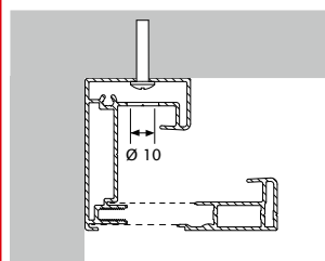
Rear mounting of the side channel Fixscreen® 85
