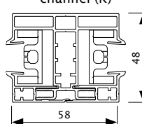
Coupling side channel (K)
