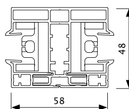
Coupling side channel (K)
