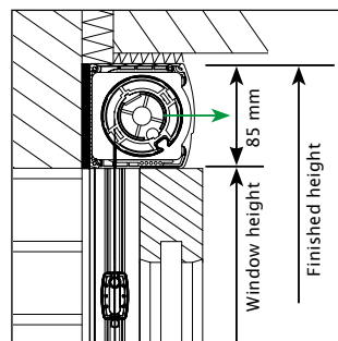
Hidden installation, reversed box, on top of the window with box, without front cover
