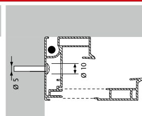
Side mounting of the side channel Fixscreen® 100 EVO
