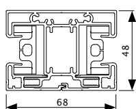
Coupling side channel (K)
