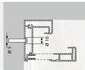
Side mounting of the side channel Fixscreen® 150 (F)
