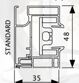
Open side channel (S)
