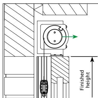
Hidden installation, with brackets, without box
