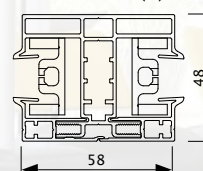
Coupling side channel (K)
